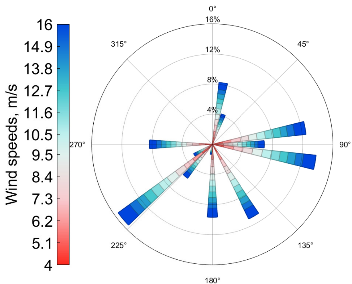
Wind Scenario 3
